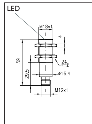
Dimensional drawing FE 18 RL
