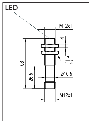
Dimensional drawing FE 12 RL
