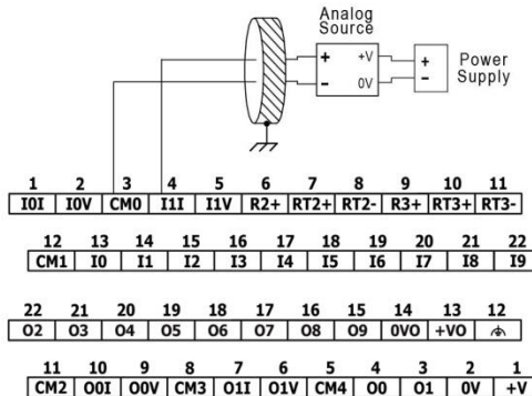
4-wire
