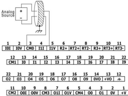
Differential
