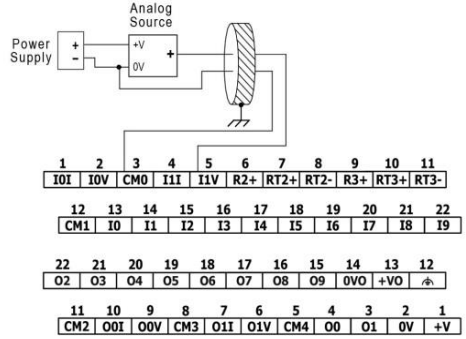
Single-ended
